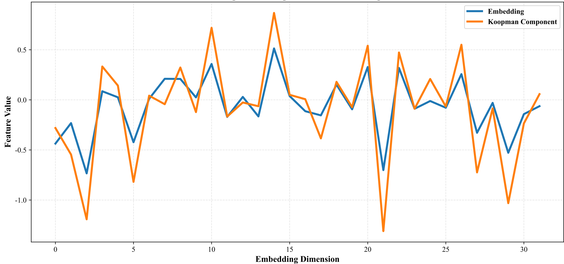
Koopman Component vs Embedding
